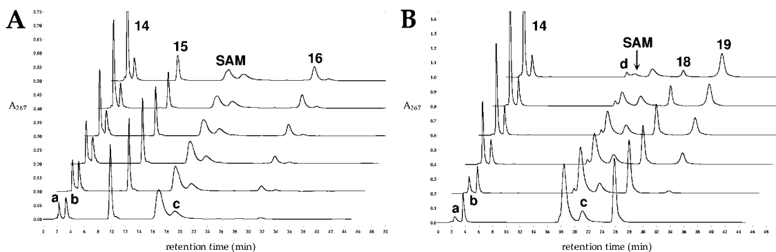
Figure 1. Representative HPLC chromatograms for stoichiometry experiments with \text{Na}_2\text{S}_2\text{O}_4 as the reductant. (A) Deamination of TDP-4-amino-4,6-dideoxy-D-glucose ( 15 ). (B) Dehydrogenation of TDP-D-quinovose ( 18 ). The bottom chromatogram in both (A) and (B) corresponds to the reaction before adding DesII. Subsequent traces are at increasing incubation times not exceeding 90 and 130 min, respectively. Peaks 14 , 16 and 19 correspond to reaction products 5'-deoxyadenosine, TDP-3-keto-4,6-dideoxy-D-glucose and TDP-3-keto-6-deoxy-D-glucose, respectively. Peaks a , b and c are contaminants in the commercial SAM. Peak d is a contaminant in the TDP-D-quinovose ( 18 ) and corresponds to deoxythymidine monophosphate. Peaks a and 14 overlap, and the correction for f_{\text{SAM}} is described in the Results and further detailed in the Supporting Information.
