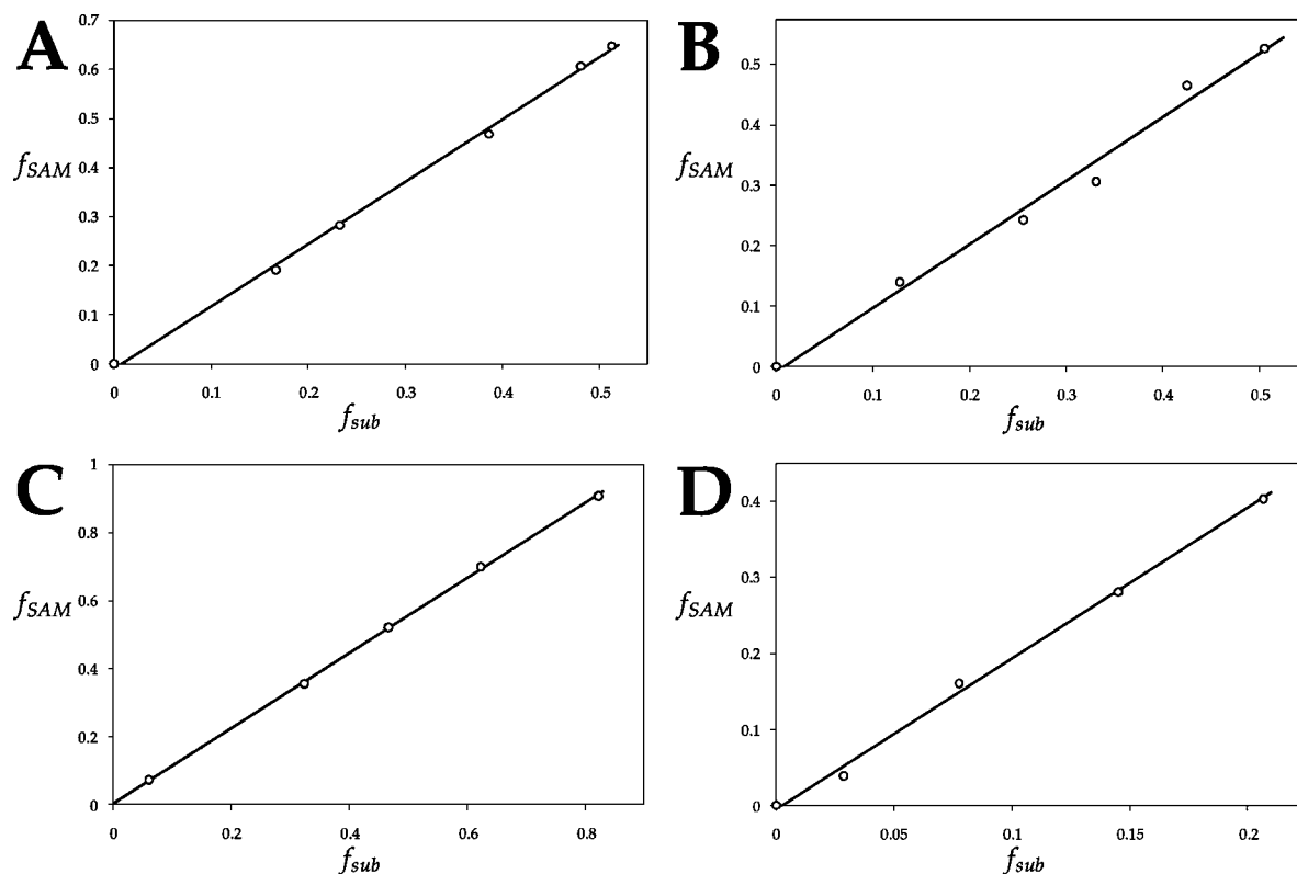
Figure 2. Representative fits of the fraction of reaction in terms of SAM, f_{\text{SAM}} , versus TDP-4-amino-4,6-dideoxy-D-glucose ( 15 ) or TDP-D-quinovose ( 18 ), f_{\text{sub}} . Trend lines are fit under the assumption of equal variance in both f_{\text{SAM}} and f_{\text{sub}} . The stoichiometry is equal to the slope divided by the correction factor, \gamma , for the given experiment. (A) Substrate 15 with \text{Na}_2\text{S}_2\text{O}_4 ( \gamma = 1.23 ). (B) Substrate 15 with FLD/FNR/NADPH ( \gamma = 1.05 ). (C) Substrate 18 with \text{Na}_2\text{S}_2\text{O}_4 ( \gamma = 1.16 ). (D) Substrate 18 with FLD/FNR/NADPH ( \gamma = 2.04 ).
