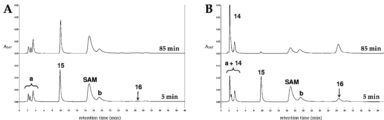
Figure 3. HPLC experiments demonstrating a requirement for a constant source of reducing equivalents in the deamination of TDP-4-amino-4,6-dideoxy-D-glucose ( 15 ) to TDP-3-keto-4,6-dideoxy-D-glucose ( 16 ) by DesII. (A) Incubation of reduced DesII with 15 at 5 and 85 min demonstrating less than 2% turnover at each time point. (B) Incubation of reduced DesII with 15 in the presence of fresh \text{Na}_2\text{S}_2\text{O}_4 at 5 and 85 min demonstrating 23 and 94% turnover in terms of 15 , respectively. Peak 14 corresponds to 5'-deoxyadenosine generated as SAM is consumed. Peaks a and b correspond to contaminants in the commercial SAM. See text for details and Figure 4 for a comparison with the dehydrogenation reaction.
