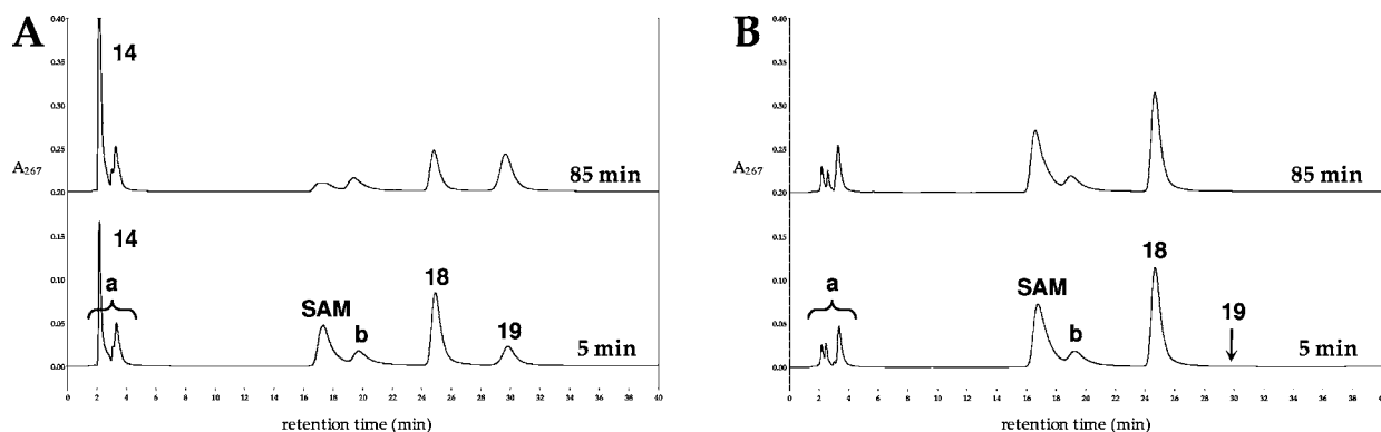
Figure 4. HPLC experiments demonstrating that a constant external source of reducing equivalents is not required for the dehydrogenation of TDP-D-quinovose ( 18 ) to TDP-3-keto-6-deoxy-D-glucose ( 19 ) by DesII. (A) Incubation of reduced DesII with 18 at 5 and 85 min demonstrating 26 and 55% reaction in terms of 18 , respectively (SAM is substoichiometric versus 18 in this experiment). (B) Incubation of nonreduced DesII with 18 in the presence of deproteinized reduced DesII filtrate at 5 and 85 min demonstrating less than 1% reaction at each time point. Peak 14 corresponds to 5'-deoxyadenosine generated as SAM is consumed. Peaks a and b correspond to contaminants in the commercial SAM. See text for details and Figure 3 for a comparison with the deamination reaction.
